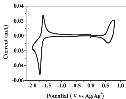
Figure 2. Cyclic voltammogram of TPA-BT-4HT film on glassy carbon electrode in an acetonitrile solution of 0.1 mol/L \text{Bu}_4\text{NPF}_6 (Bu = butyl) with a scan rate of 100 mV/s.
